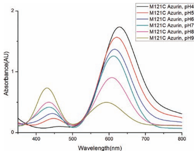
Figure 3. UV–visible spectrum for Met121Cys azurin at varying pH values from 4–9 in UB buffer (see Experimental Section).
