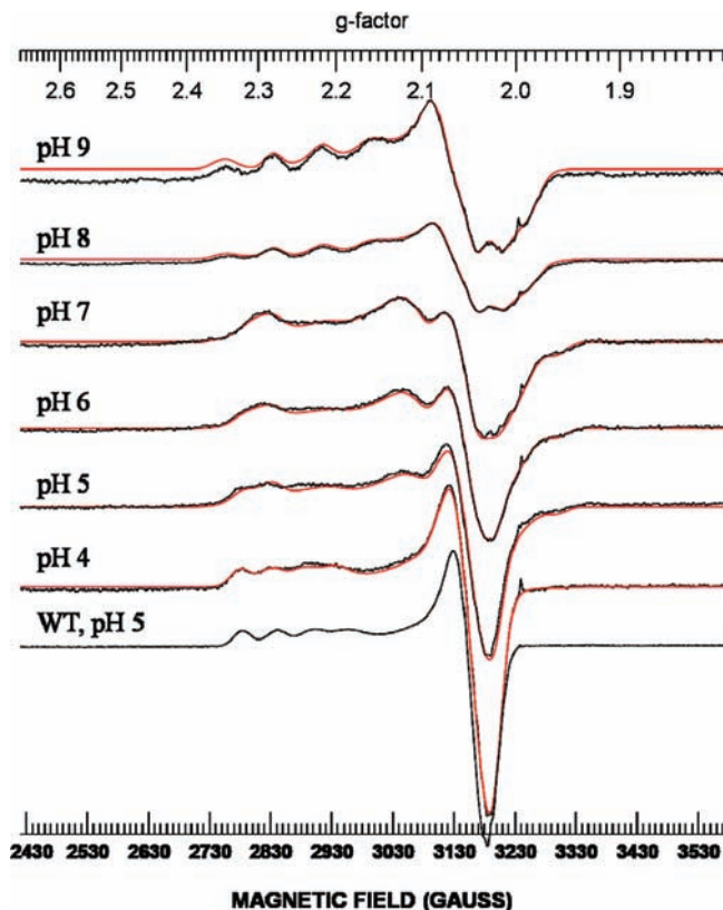
Figure 4. X-band EPR spectra of Met121Cys azurin at different pH values. The EPR spectra are in black while the simulated spectra are in red. X-band experimental conditions: microwave frequency, 9.04 GHz; power, 0.2 mW; modulation amplitude 5 G, time constant, 32 ms; sweep time, 60 s; number of scans, 10; gain, 8000; temperature, 29 K. The spike at g = 2.0 is an artifact of the EPR tubes used.
