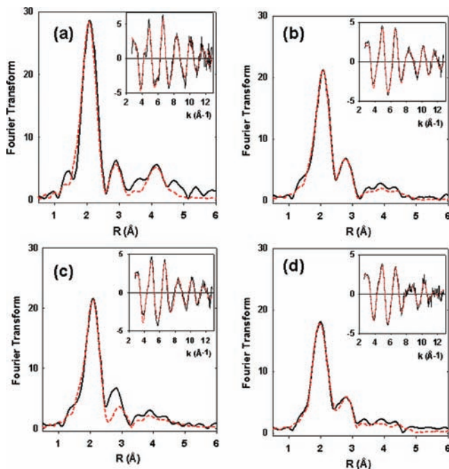
Figure 7. Fourier transform and EXAFS (inset) for the WT azurin and Met121Cys and Met121Hcy variants. Experimental data are shown as solid black lines, and the simulation is shown by dashed red lines. Parameters used to fit the data are listed in Table 2. (a) WT azurin at pH 5.0. (b) Best fit of Met121Cys variant at pH 7 (bolded in Table 2) with one short (2.17 Å) and one long (2.74 Å) Cu–S interaction. (c) Best fit of Met121Cys variant at pH 7, obtainable using only the short Cu–S distance; (d) Met121Hcy variant at pH 7.
