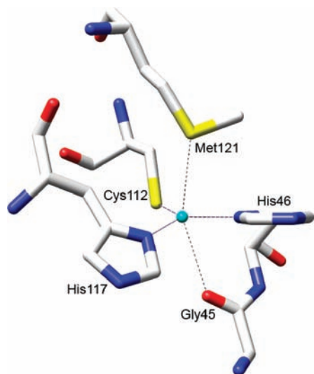
Figure 1. Type 1 copper site in Pseudomonas aeruginosa azurin.
