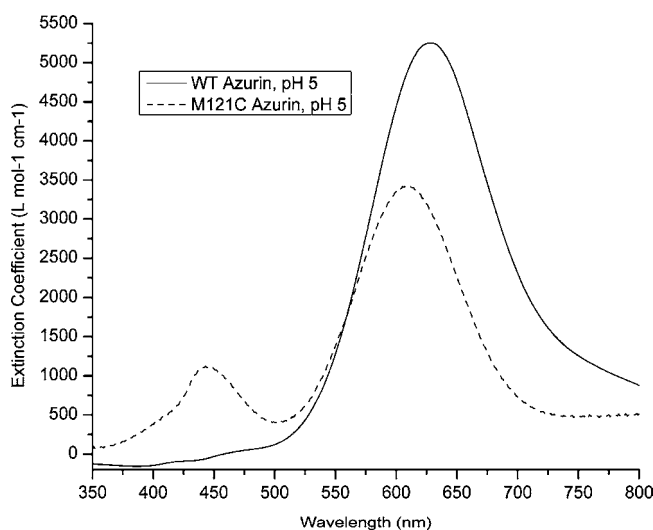
Figure 2. UV–visible spectrum for Met121Cys azurin at pH 5 in UB buffer (see Experimental Section) and comparison with WT azurin.
